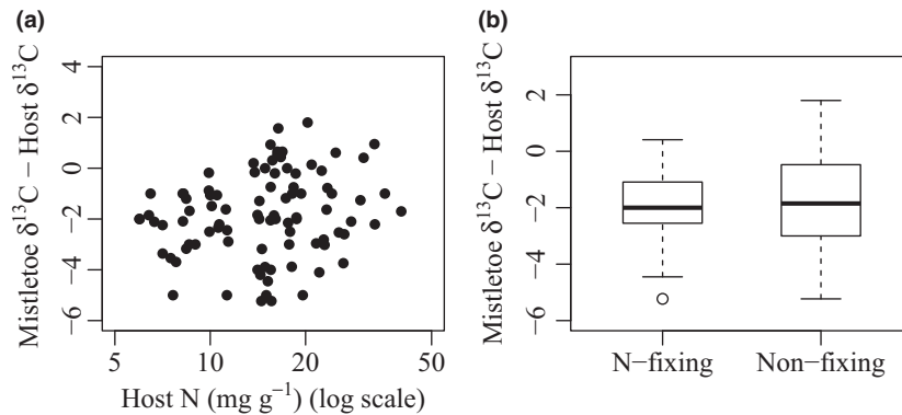
Fig. 3. (a) Mistletoe to host difference in \delta^{13}\text{C} in relation to host leaf N concentration ( r^2 = 0.03 , P = 0.08 ); and (b) pairwise comparison between mistletoe to host difference in \delta^{13}\text{C} in N-fixing ( n = 19 ) and non-fixing hosts ( n = 71 ; t = -0.69 , P = 0.49 ).
